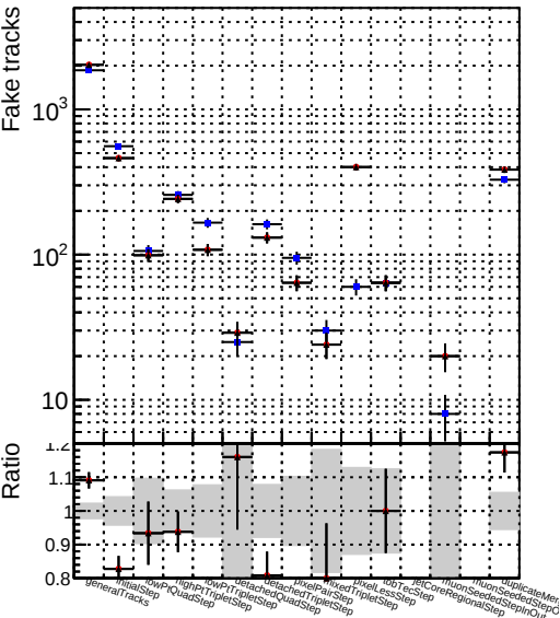
Number DQM_mkFit_SoftQCD-updated DQM_mkFit_SoftQCD-DNNsqcd100
