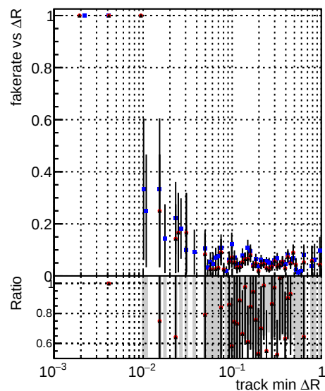
Legend for Fake rate vs \Delta R , Duplicates Rate vs \Delta R , and Pileup rate vs \Delta R : DOM_CKF_softQCD (blue squares) DOM_mkFit_SoftQCD-updated (red circles) DOM_mkFit_SoftQCD-DNNsqcd100 (black triangles)
