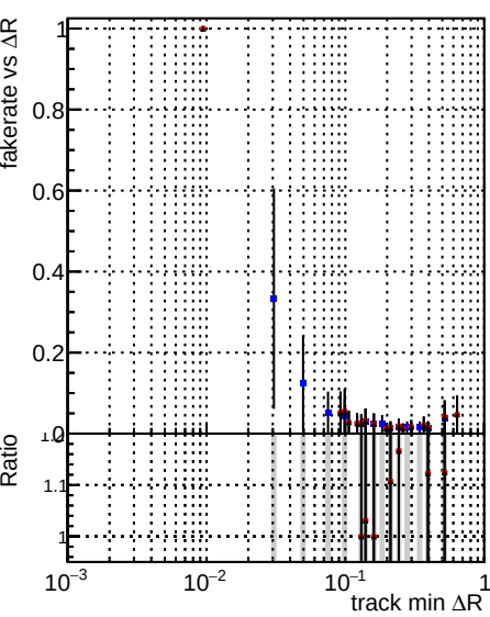
Fake rate vs ΔR(track, jet) DQM_CKF_softQCD DQM_mkFit_SoftQCD-updated DQM_mkFit_SoftQCD-DNNsqcd100
