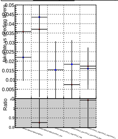
Fake rate vs. DOM CKF softQCD DOM mktFit softQCD-DNNsqcd100 DOM mktFit softQCD-DNNsqcd100
