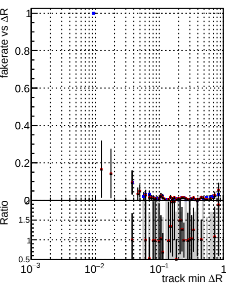
Fake rate vs \Delta R(\text{track, jet}) Legend: DOM_CKF_softQCD (blue line with dots) DOM_mkFit_SoftQCD-updated (red line with dots) DOM_mkFit_SoftQCD-DNNsqcd100 (black line with dots)
