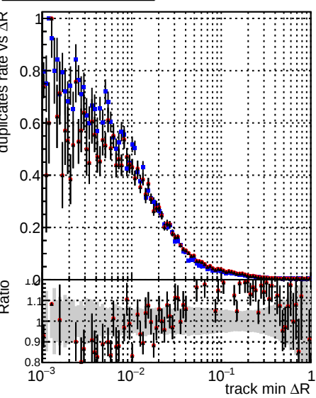
DOM_CKF_softQCD DOM_mkFit_SoftQCD-updated DOM_mkFit_SoftQCD-DNNsqcd100
