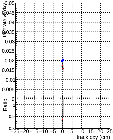
Legend for Fake rate vs dxy, Duplicates Rate vs Dxy, and Pileup rate vs dxy: DOM CKF softOCD (blue) DOM CKF softOCD-updated (red) DOM mktFit softOCD (black) DOM mktFit softOCD-BNNsqcd100 (grey)
