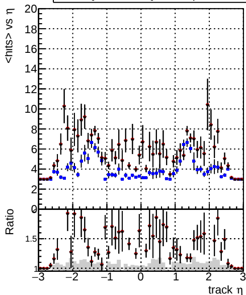
mean hit — DQM_CKF_softQCD — DQM_mkFit_SoftQCD-updated — DQM_mkFit_SoftQCD-DNNsqcd100
