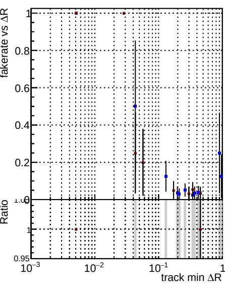
Fake rate vs ΔR(track, jet) Legend: DQM_CKF_softQCD (blue dots) DQM_mkFit_SoftQCD-updated (red dots) DQM_mkFit_SoftQCD-DNNsqcd100 (black dots)
