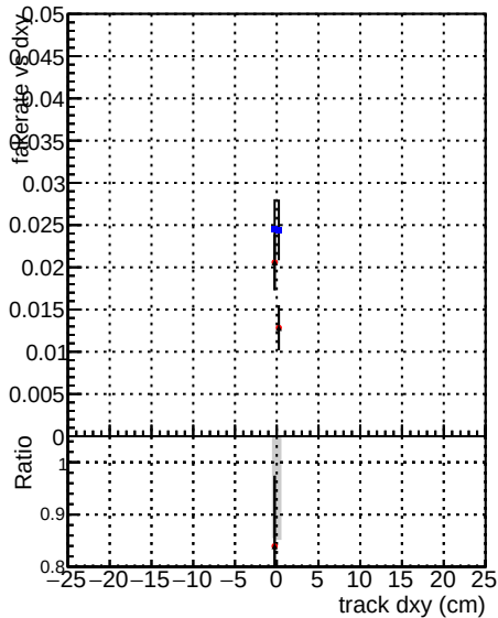
Legend: DOM CKF softQCD DOM CKF softQCD-updated DOM mktFit softQCD-BNNsgcd100
