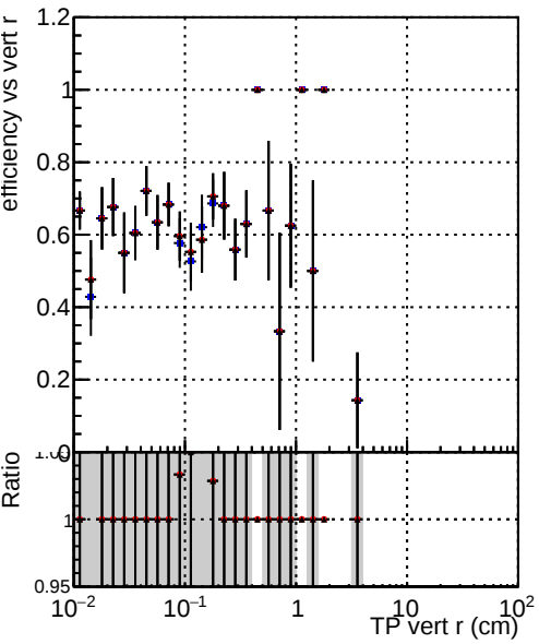
Efficiency vs vertpos DQM_CKF_softQCD DQM_mkFit_SoftQCD-updated DQM_mkFit_SoftQCD-DNNsqcd100
