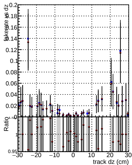
DOM CKF softOCD BQM mktFit softOCD-updated BQMnsqcd100
