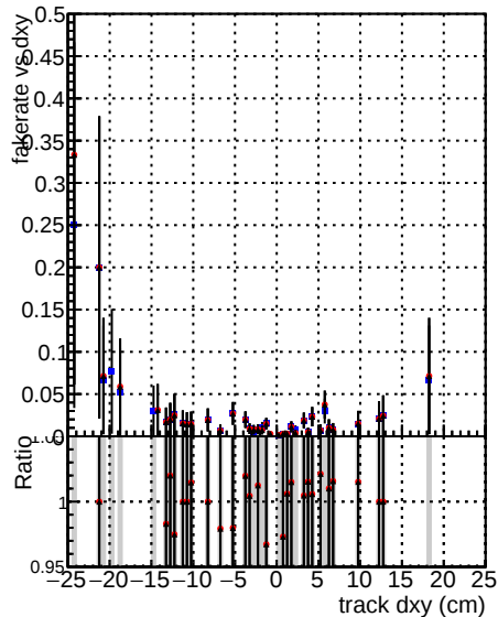
DOM CKF softOCD BQM mktFit softOCD-updated BQMnsqcd100
