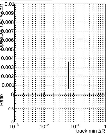
Legend: DOM_CKF_softQCD (grey line with markers) DOM_mkFit_SoftQCD-updated (red line with markers) DOM_mkFit_SoftQCD-DNNsqcd100 (black line with markers)
