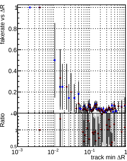
Fake rate vs \Delta R(\text{track}, \text{jet}) DOM_CKF_softQCD DOM_mkFit_SoftQCD-updated DOM_mkFit_SoftQCD-DNNsqcd100
