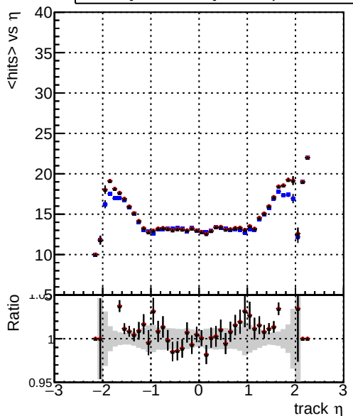
mean hits vs \eta — DQM_CKF_softQCD — DQM_mkFit_SoftQCD-updated — DQM_mkFit_SoftQCD-DNNsqcd100
