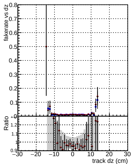
— DOM CKF softQCD — DOM CKF softQCD-updated — DOM mktFit softQCD-BNNsqcd100
