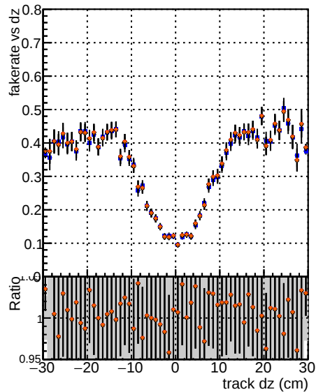
Fake rate vs dz DGM GKE softQCD DGM+GKE+softQCD+updated DGM+GKE+softQCD+updated+100 DGM+GKE+softQCD+updated+100+100 DGM+GKE+softQCD+updated+100+100+100
