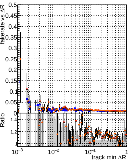
Fake rate vs \Delta R(\text{track, jet}) Legend: DOM CKE softQCD DOM mktfit softQCD DOM mktfit softQCD-BNN DOM mktfit softQCD-BNN-100 DOM mktfit softQCD-BNN-1000
