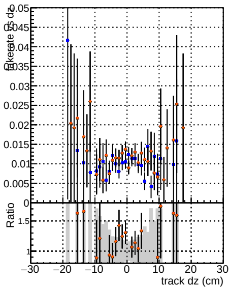
Fake rate vs d DOM CKE softOCD DOM+CKE softOCD+updated softOCD+DNN softOCD+DNN+all
