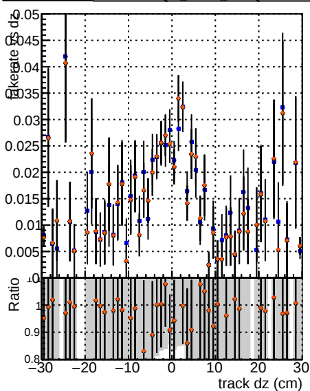
Fake rate vs d DOM CKE softOCD DOM+CKE softOCD+updated softOCD+DNN softOCD+DNN+all
