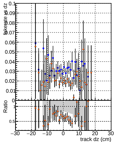
Fake rate vs d —●— BGM GKE softQSP —●— BGM GKE softQSP updated —●— BGM GKE softQSP d100 —●— BGM GKE softQSP d100 —●— BGM GKE softQSP d100
