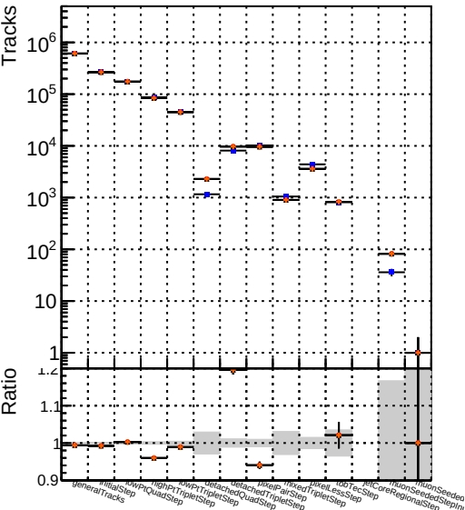
Number —■— DQM_CKF_softQCD —●— DQM_mkFit_SoftQCD-updated —★— DQM_mkFit_SoftQCD-DNNsqcd10 —◆— DQM_mkFit_SoftQCD-DNNalliters
