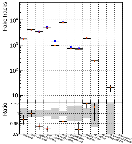
Number of tracks vs collection Legend: DQM_CKF_softQCD DQM_mkFit_SoftQCD-updated DQM_mkFit_SoftQCD-DNNsqcd100 DQM_mkFit_SoftQCD-DNNalliters
