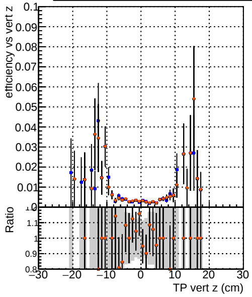
Efficiency vs vert z DOM_CKF_SoftQCD DOM_mkFit_SoftQCD-updated DOM_mkFit_SoftQCD-DNNsqcd100 DOM_mkFit_SoftQCD-DNNalliters
