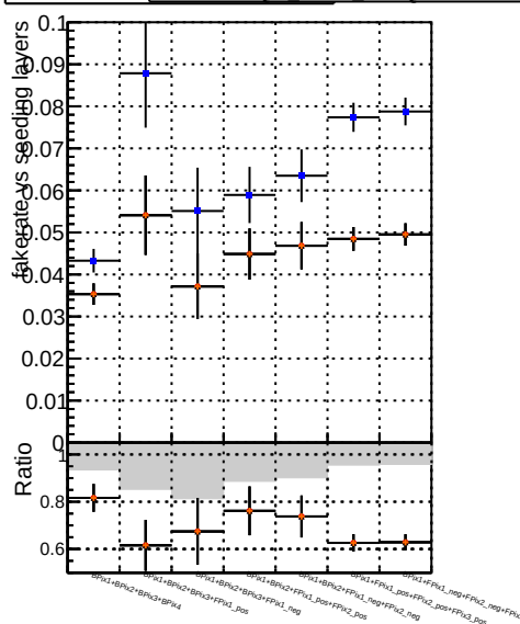
Fake rate vs. DOM GKE softQCD BNN
