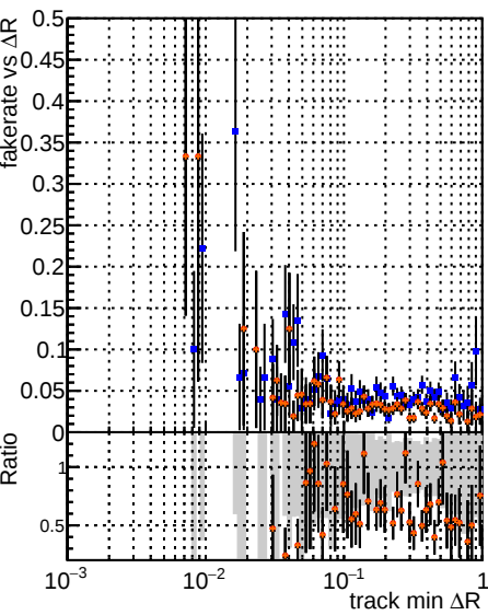
Fake rate vs \Delta R(\text{track}, \text{jet}) Legend: DOM CKE softQCD mkrfit softQCD-updated softQCD-100 BNN filters
