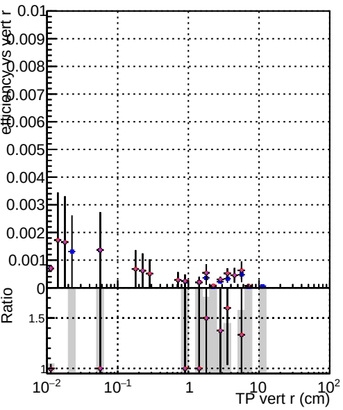
Efficiency vs vertpos DOM CKE SoftOCD DOM mkFit SoftOCD-updated DOM mkFit SoftOCD-updated-newPLDNN DOM mkFit SoftOCD-updated-TTbarDNN DOM mkFit SoftOCD-updated-DNNsqcd13
