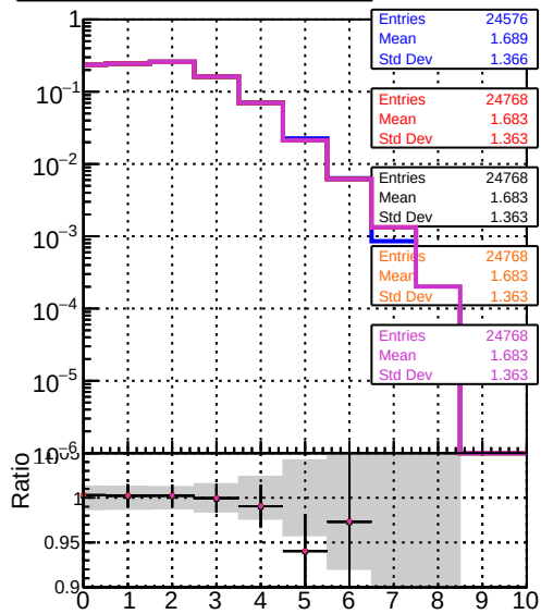
mean hits DOM CKE SortOCB DOM mkFit SortOCB-updated newPLDNN DOM mkFit SortOCB-updated TTbarDNN DOM mkFit SortOCB-updated DNNsqcd13
