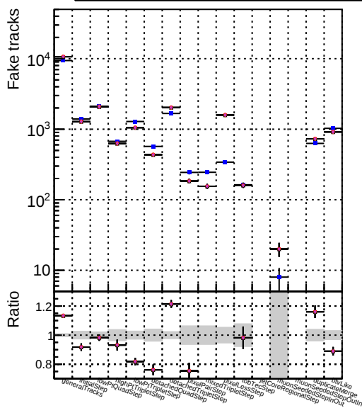
Number Model Method Dataset Model Method Dataset 1 DOM mkFit SoftQCD-updated newPLDNN 2 DOM mkFit SoftQCD-updated TTbarDNN 3 DOM mkFit SoftQCD-updated DNNsgcd13
