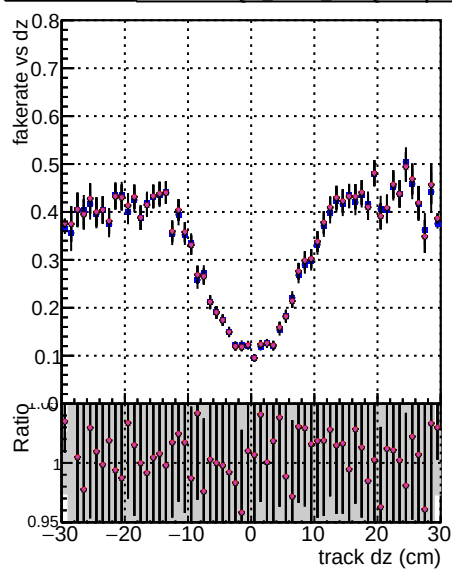
DOM CKF softQCD DOM CKF hardQCD DOM CKF softQCD+hardQCD DOM CKF softQCD+hardQCD+updated DOM CKF softQCD+hardQCD+updated+NN+sc13 DOM CKF softQCD+hardQCD+updated+NN+sc13+NN+sc13
