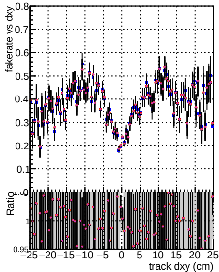
DOM CKF softQCD DOM CKF hardQCD DOM CKF softQCD+hardQCD DOM CKF softQCD+hardQCD+updated DOM CKF softQCD+hardQCD+updated+NN+sc13 DOM CKF softQCD+hardQCD+updated+NN+sc13+NN+sc13
