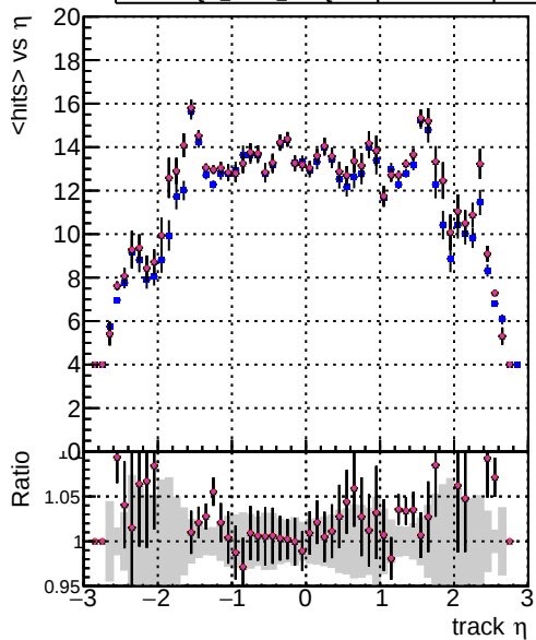
Legend: DQM_CKE_SortOCB, DQM_mktFit_SortOCB-updated, DQM_mktFit_SortOCB-updated-newPLDNN, DQM_mktFit_SortOCB-updated-TTbarDNN, DQM_mktFit_SortOCB-updated-DNNsqc13 mean hits
