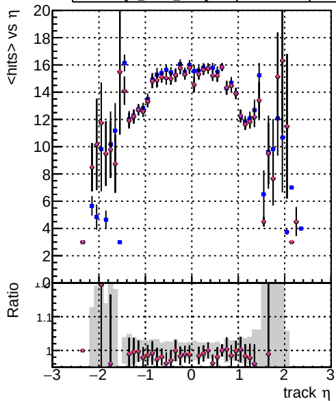
mean hit DOM CKE SortOCB DOM mkFit SortOCB-updated DOM mkFit SortOCB-updated-newPLDNN DOM mkFit SortOCB-updated-TTbarDNN DOM mkFit SortOCB-updated-DNNsqc13
