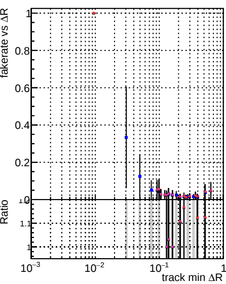
Fake rate vs ΔR(track, jet) for various models: DQM, GKE, softQCD, DNN, GCD, updated-DNN, softQCD+DNN, updated-DNN+softQCD, newPLDNN, and GCD13.
