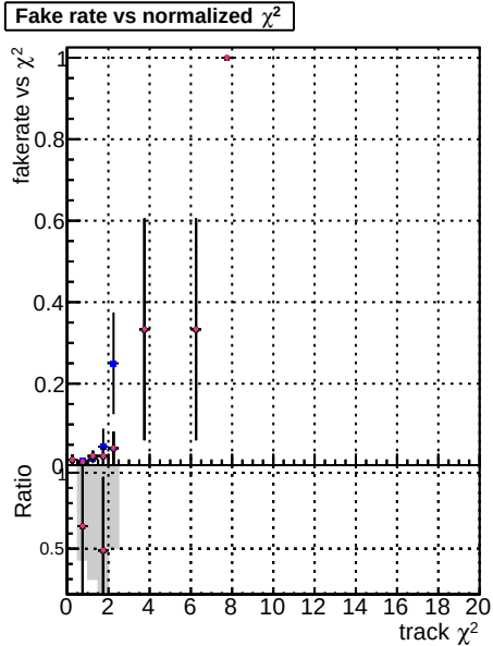
Fake rate vs. DOM GKF softQCD DOM GKF softQCD-Updated DOM GKF softQCD-Updated-BNN DOM GKF softQCD-Updated-BNN-Scal3
