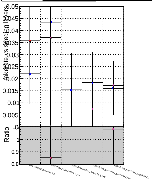
Fake rate vs. DOM GKF softQCD DOM GKF softQCD-Updated DOM GKF softQCD-Updated-BNN DOM GKF softQCD-Updated-BNN-Scal3
