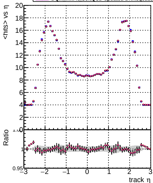
mean hits vs \eta DOM CKE SortOCB DOM mkFit SortOCB-updated newPLDNN DOM mkFit SortOCB-updated TTbarDNN DOM mkFit SortOCB-updated DNNsqc13
