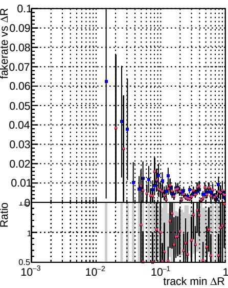
Fake rate vs \Delta R(\text{track, jet}) DQM GKE softQCD DNN updated newPLDNN DNNsqcd13
