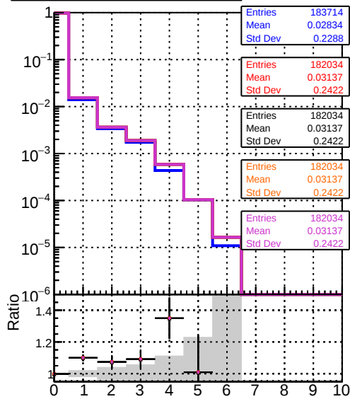
Legend: DOM CKE SortOCB DOM mkFit SortOCB-updated DOM mkFit SortOCB-updated newPLDNN DOM mkFit SortOCB-updated TBarDNN DOM mkFit SortOCB-updated DNNsqc13 mean hits
