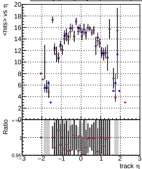
mean hit DOM CKE SortOCB DOM mkFit SortOCB-updated DOM mkFit SortOCB-updated-newPLDNN DOM mkFit SortOCB-updated-TTbarDNN DOM mkFit SortOCB-updated-DNNsgcd13
