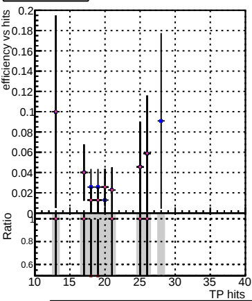
Efficiency vs hit DOM_CKF_softQCD DOM_mkFit_SoftQCD-updated DOM_mkFit_SoftQCD-updated-newPLDNN DOM_mkFit_SoftQCD-updated-TTbarDNN DOM_mkFit_SoftQCD-updated-DNNsqcd13
