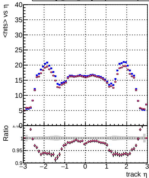
mean hits DOM CKE SoftOCB DOM mkFit SoftOCB-updated DOM mkFit SoftOCB-updated newPLDNN DOM mkFit SoftOCB-updated TbarDNN DOM mkFit SoftOCB-updated DNNsqc13
