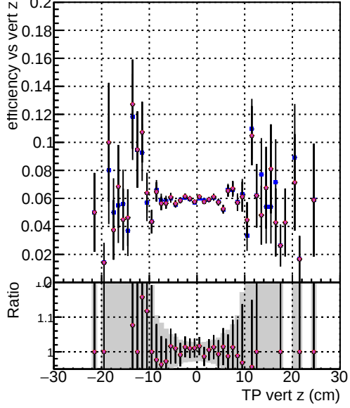
Efficiency vs vert z — DOM CKE SortOCB — DOM mkFit SortOCB — DOM mkFit SortOCB-updated — DOM mkFit SortOCB-updated-newPLDNN — DOM mkFit SortOCB-updated-TTbarDNN — DOM mkFit SortOCB-updated-DNNsqcd13
