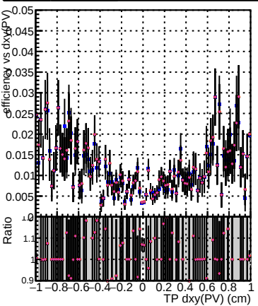
Efficiency vs Dxy(PV) DOM_CKF_SoftQCD DOM_mkFit_SoftQCD-updated DOM_mkFit_SoftQCD-updated-newPLDNN DOM_mkFit_SoftQCD-updated-TTbarDNN DOM_mkFit_SoftQCD-updated-TTbarDNN25
