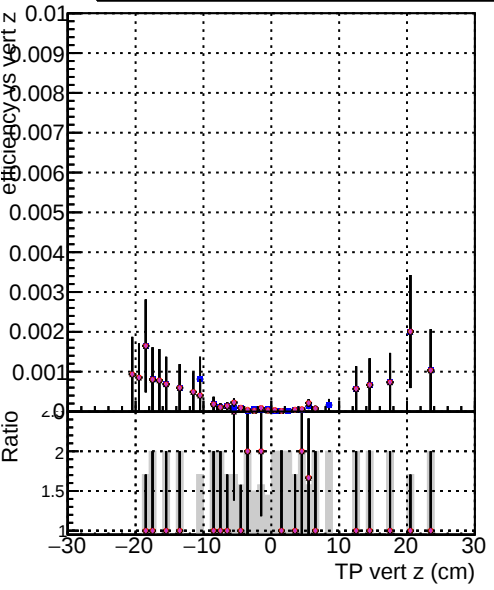
Efficiency vs vertpos DOM CKE SoftOCD DOM mkFit SoftOCD-updated DOM mkFit SoftOCD-updated-newPLDNN DOM mkFit SoftOCD-updated-TTbarDNN DOM mkFit SoftOCD-updated-TTbarDNN25
