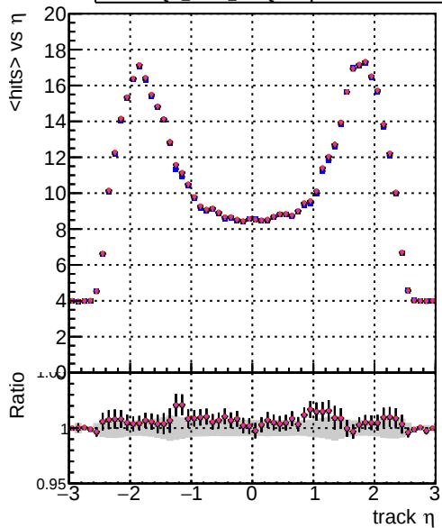
mean hit DOM_CKE_SortOCB DOM_mkFit_SortOCB-updated DOM_mkFit_SortOCB-updated-newPLDNN DOM_mkFit_SortOCB-updated-TTbarDNN25
