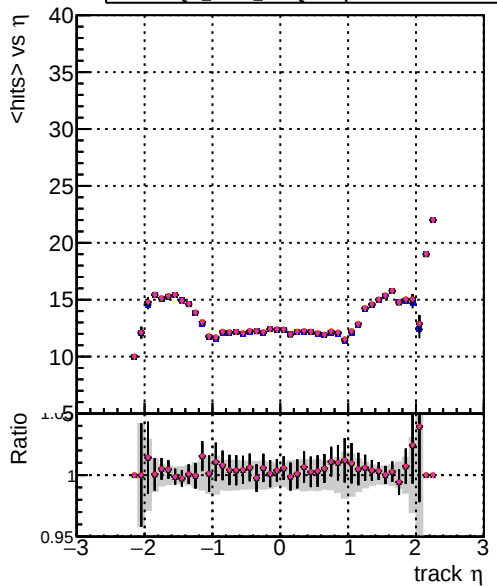
mean hits DOM CKE SortOCB DOM mkFit SortOCB-updated DOM mkFit SortOCB-updated newPLDNN DOM mkFit SortOCB-updated T1barDNN25
