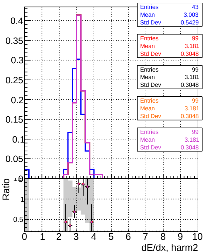
Legend: DOM_CKF_SoftOCD (blue line) DOM_mkFit_SoftOCD-updated (red line) DOM_mkFit_SoftOCD-updated-newPLDNN (black line) DOM_mkFit_SoftOCD-updated-TTbarDNN (orange line) DOM_mkFit_SoftOCD-updated-TTbarDNN25 (purple line)
