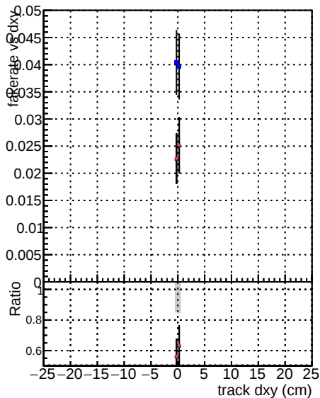
Fake rate vs d DOM GKE softGPD DOM GKE softGPD-updated DOM GKE softGPD-updated-new DOM GKE softGPD-updated-TTbarDNN25
