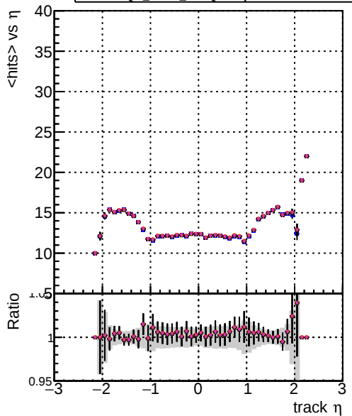
mean hits vs \eta DOM CKE SortOCB DOM mkFit SortOCB-updated DOM mkFit SortOCB-updated newPLDNN DOM mkFit SortOCB-updated TTbarDNN25
