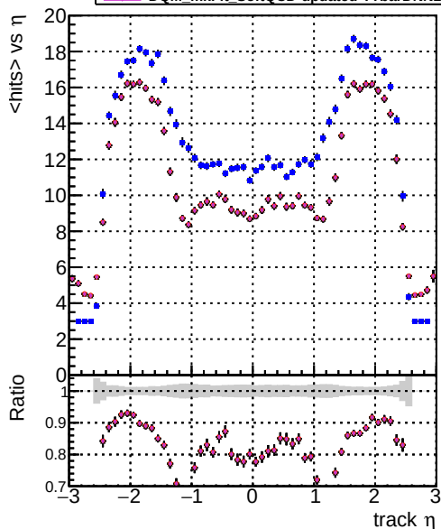
mean hit DOM CKE SortOCB DOM mkFit SortOCB-updated newPLDNN DOM mkFit SortOCB-updated TTbarDNN25 DOM mkFit SortOCB-updated TTbarDNN
