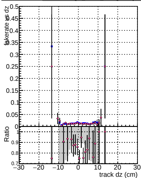
DOM GKE softQCD DOM GKE softQCD-updated DOM GKE softQCD-updated-new DOM GKE softQCD-updated-new+DNN25 DOM GKE softQCD-updated-new+DNN25
