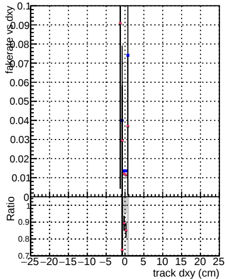
DOM GKE softQCD DOM GKE softQCD-updated DOM GKE softQCD-updated-new DOM GKE softQCD-updated-new+DNN25 DOM GKE softQCD-updated-new+DNN25
